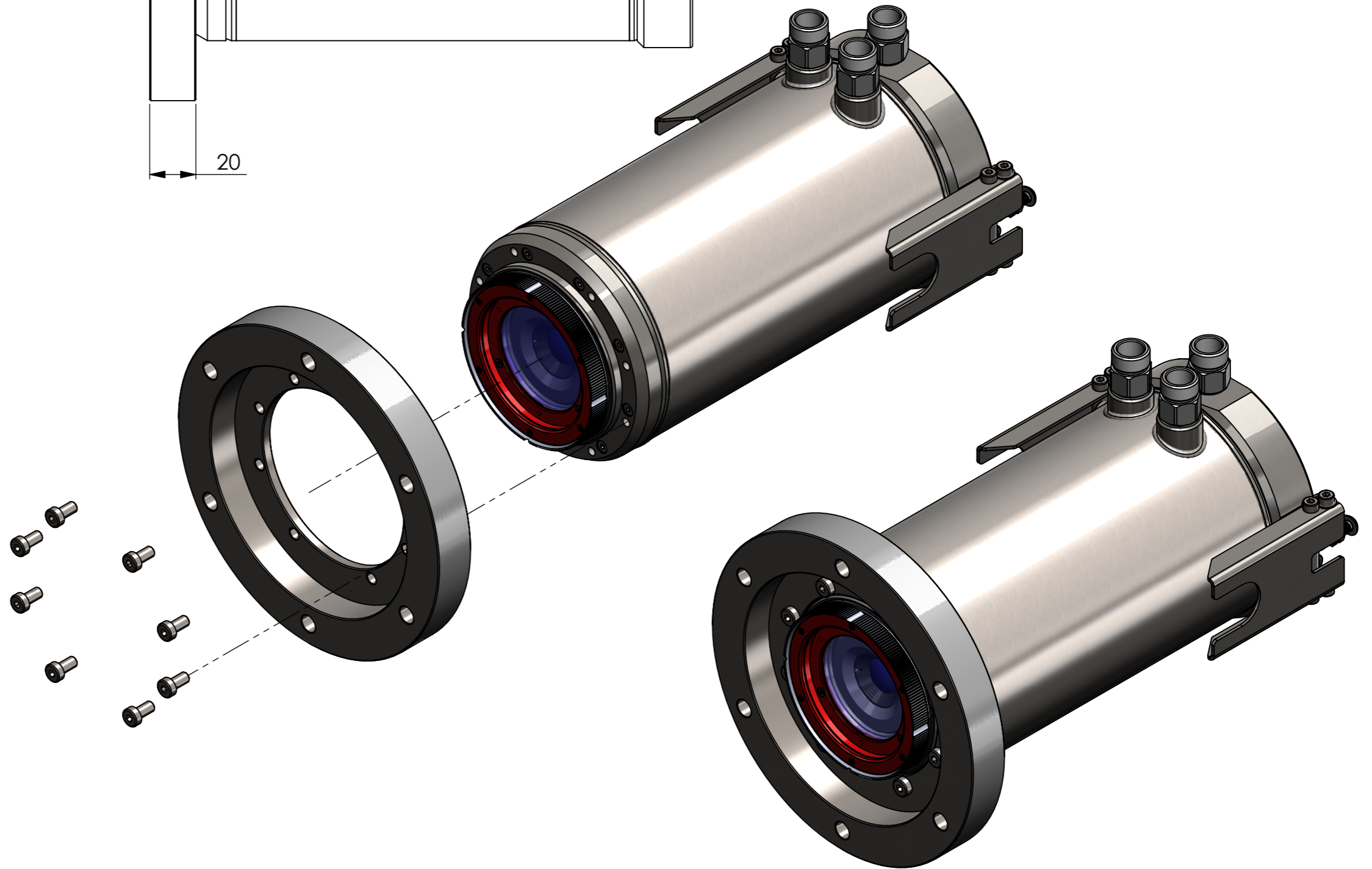
Mounting flange for Cooling-jacket-Advanced
